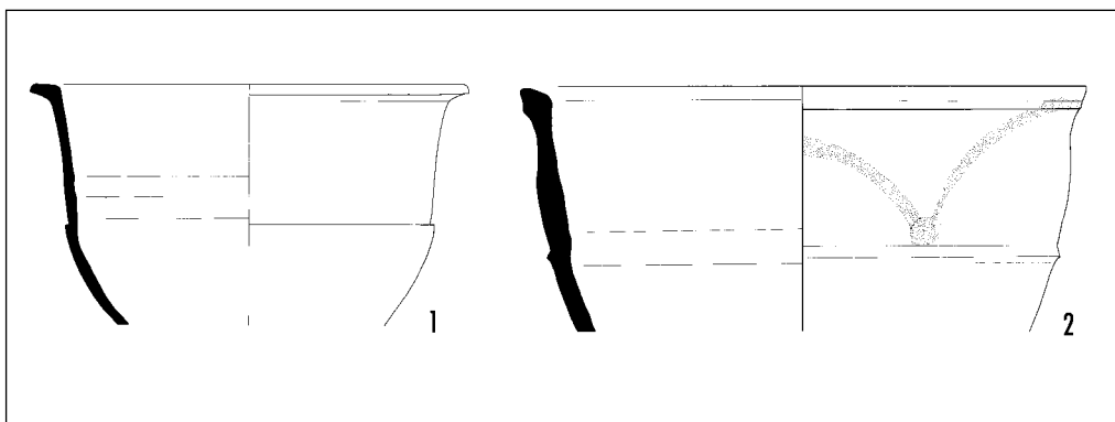
Fig. 1. Mareotic carinated bowls. Scale 1:4 (Drawing G. Majcherek)
