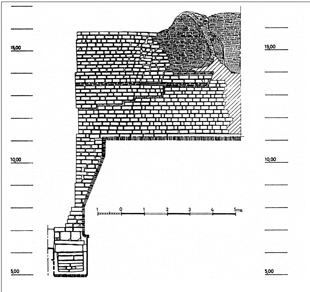
Fig. 8. Cisterns. Restored corner of the northern facade (Drawing W. Kolqataj)
