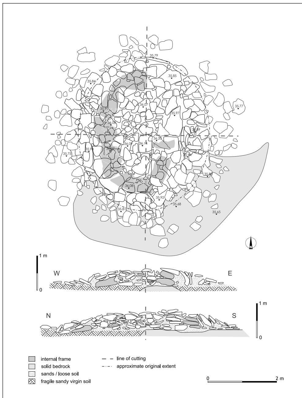
Fig. 4. SB 69: general plan including outline of the inner kerb (inside dismantled quadrants); bottom, N-S and E-W cross-sections (Drawing and digitizing E. Mizak, editing Ł. Rutkowski)
