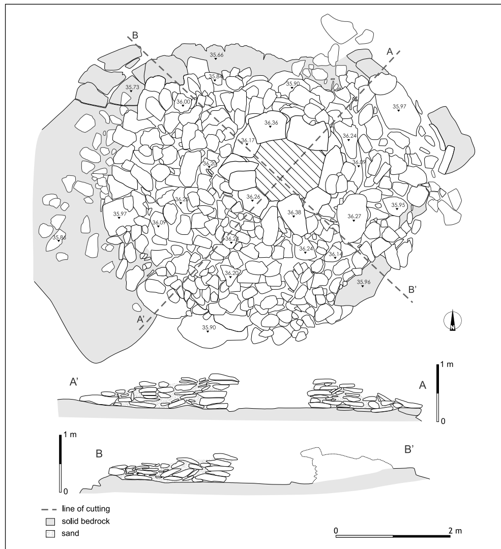
Fig. 7. SB 70: plan and cross-sections (Drawing and digitizing E. Mizak)
